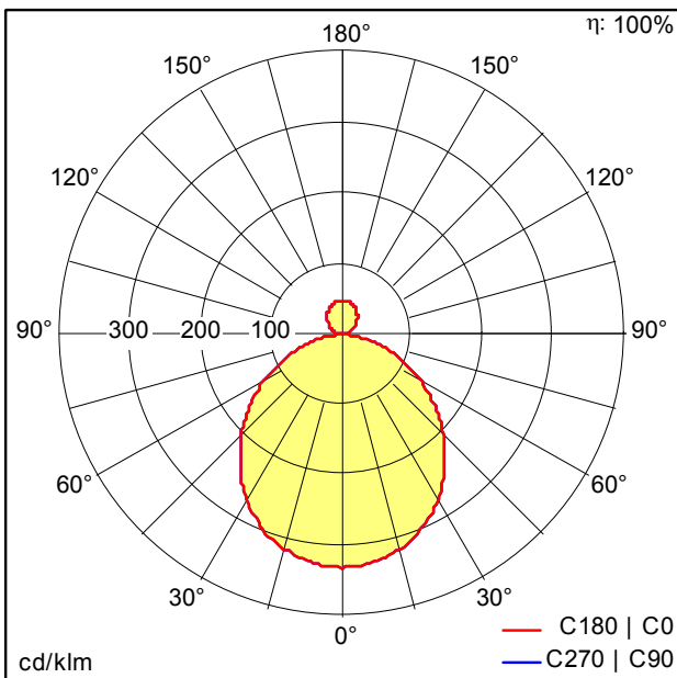
D39348AA_ONDA2_A_AV_D590_LED2500-840_SR_BK.Idt
