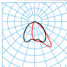
Jovie 70I-AM3L-SLR3/15000-740 12G1 ET TX195580 ■ C0 - C180 ■ C90 - C270 DIN 5040: A50 UTE: 1,00 D CEN Flux Code: 59 89 100 100 100
