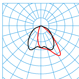
Jovie 70I-AM3L-SLR3/15000-740 12G1 ET (CLO initial value) TX300279 ■ C0 - C180 ■ C90 - C270 DIN 5040: A50 UTE: 1,00 D CEN Flux Code: 59 89 100 100 100
