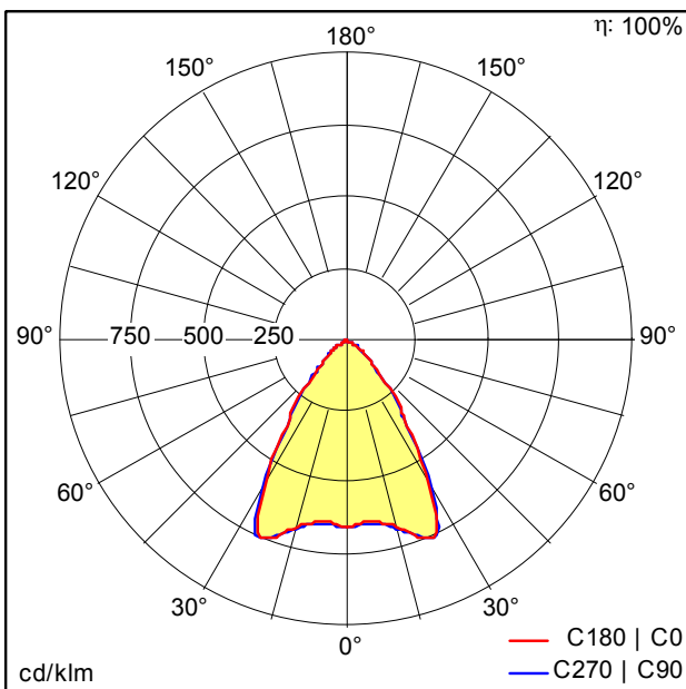
D42326AA_TECTON_MIRL_LED4000-830_L1500_LDO_BK.Idt
