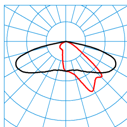
Jovie 50-AB2L-LRA/2200-730 4G1 ET (CLO initial value) TX300266 ■ C0 - C180 ■ C90 - C270 DIN 5040: A30 UTE: 1,00 G CEN Flux Code: 34 71 96 100 100
