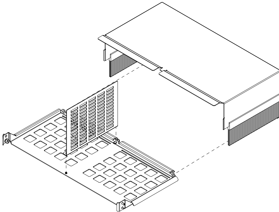
ISO VIEW
