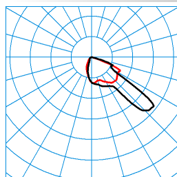
LIQ 50N-FR1L/5600-740 6G1 ET (CLO end value) TX278118
