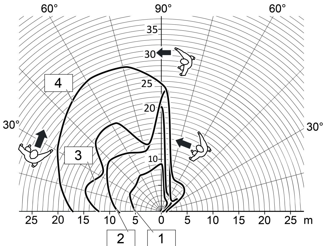
Figure 14: Range with tangential direction of motion, device variant 1.10 m, only one sensor active
