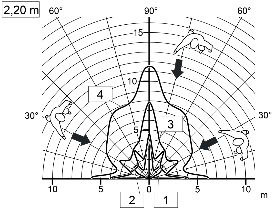
Figure 6: Range with radial direction of motion, mounting height 2.20 m
