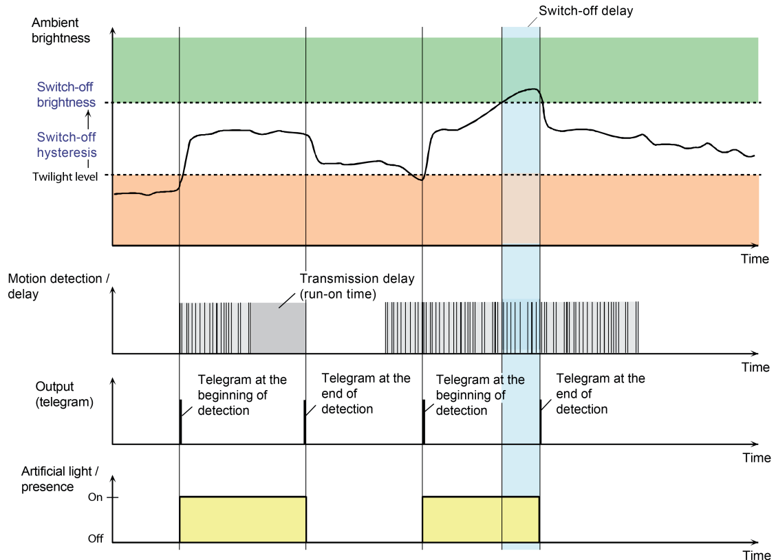
Figure 29: Brightness and motion evaluation with the detector with switch-off brightness
