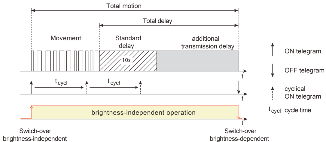
Figure 46: Total motion with motion detection, standard delay and additional transmission delay
