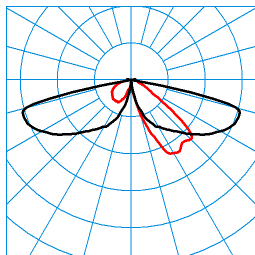
CS 19 100-AB2L-SLR1/5100-730 4G1S ET (CLO initial value) TX300051 ■ C0 - C180 ■ C90 - C270 DIN 5040: A20 UTE: 1,00 l CEN Flux Code: 27 65 96 100 100 0 0 0 0
