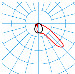
Jovie 50I-AM2L-SLR3/4200-730 4G1 ET (CLO end value) TX300748 ■ C0 - C180 ■ C90 - C270 DIN 5040: A40 UTE: 1,00 F CEN Flux Code: 47 91 100 100 100
