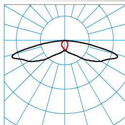
LIQ 50N-SB3L-SLR2/2200-730 2G1 ET (CLO end value) TX277731 ■ C0 - C180 ■ C90 - C270 DIN 5040: A30 UTE: 1,00 l CEN Flux Code: 31 64 92 100 100
