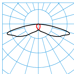
LIQ 50N-SB3L-SLR2/2200-730 2G1 ET (CLO initial value) TX277817 ■ C0 - C180 ■ C90 - C270 DIN 5040: A30 UTE: 1,00 l CEN Flux Code: 31 64 92 100 100
