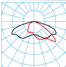
LnPlus 60-AB7L/26000-727 24G1 ETDD (CLO end value) TX390083 ■ C0 - C180 ■ C90 - C270 DIN 5040: A30 UTE: 1,00 G CEN Flux Code: 35 73 98 100 100
