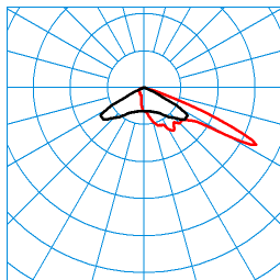
LnPlus 60-AM19L-SLR2/26000-722 24G1 ET (CLO initial value) TX390098 ■ C0 - C180 ■ C90 - C270 DIN 5040: A30 UTE: 1,00 J CEN Flux Code: 28 76 99 100 100
