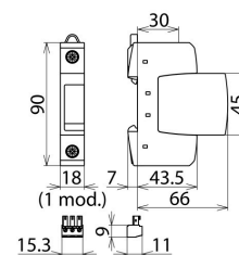
Dimensions DG S 150 FM
