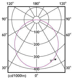
Downlight DN065C G3 LDNR CCT D150 RD-LDD
