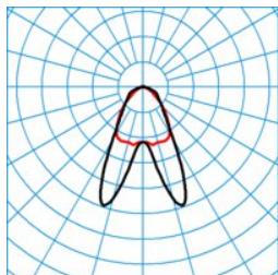
7850 HE LDAN80 865 L150 3 50 ■ C0 - C180
