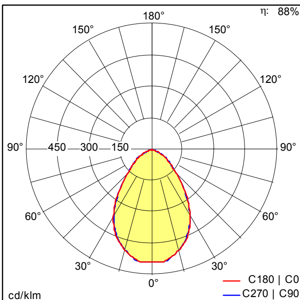
ST7345_M.Idt
