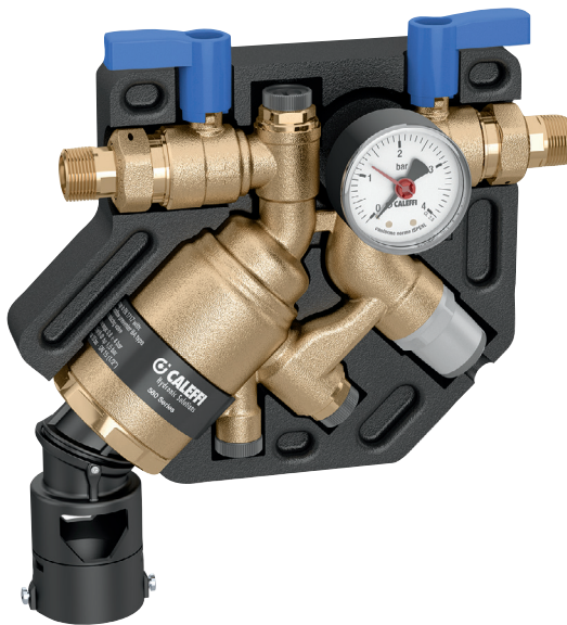
580010 DN 15 (1/2")
