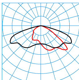
Jovie 70-AB7L-ML/165-240-740 24G1 ETDD (CLO initial value) TX271512 ■ C0 - C180 ■ C90 - C270 DIN 5040: A30 UTE: 1,00 G CEN Flux Code: 35 73 97 100 100
