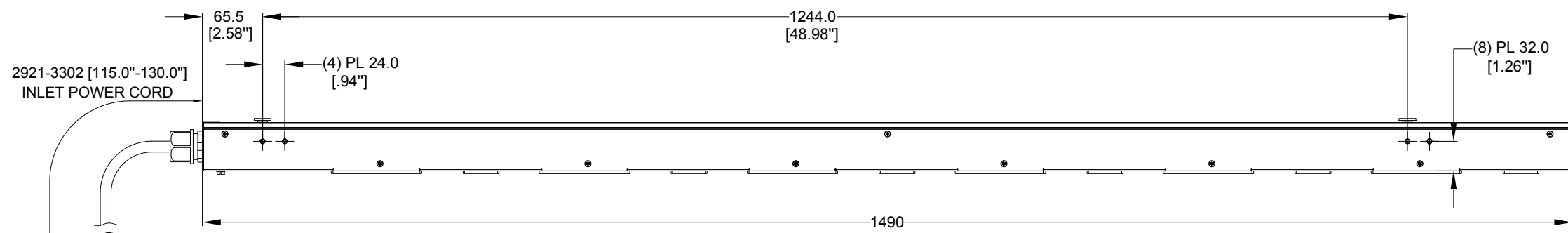
TOP VIEW
