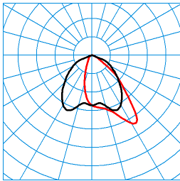
Jovie 70I-AM3L-LRA/24000-730 24G1 ET (CLO end value) TX301038 ■ C0 - C180 ■ C90 - C270 DIN 5040: A50 UTE: 1,00 D CEN Flux Code: 59 89 100 100 100
