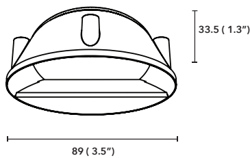
DTRW50 Downlight Trim Round Wall Wash
