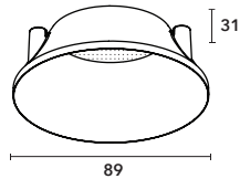
DTRFW50 Downlight Trim Round Fixed IP44 (Solite Lens)
