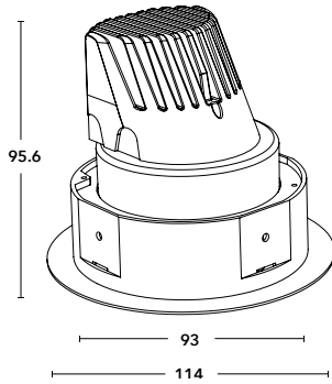
DERF50-T Downlight Light Engine Round Fixed Trimmed
