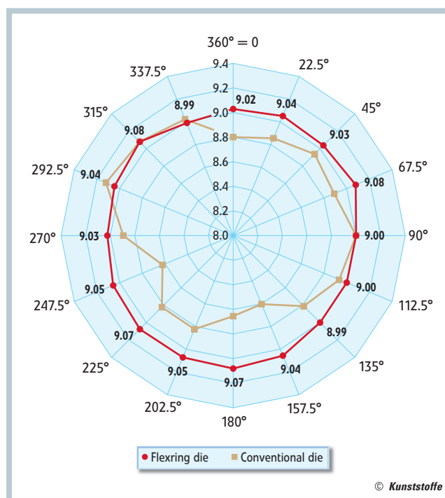
Fig. 3. Wall thickness distribution over the circumference of the die achieved with a Flexring die through local optimization of the flow channel gap (pipe geometry: 110 x 9 mm)
