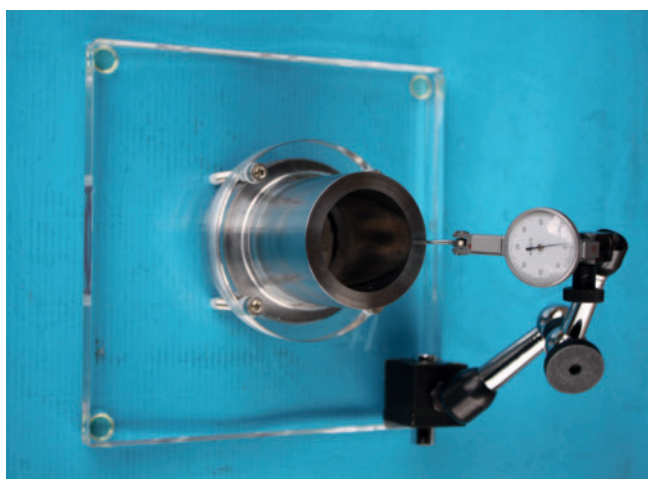
Fig. 1. Exhibition model for demonstrating the benefits of tilting die technology. The four flange bolts are used not only for clamping purposes, but also to tilt the die (photos without fig. 4: Gross)
