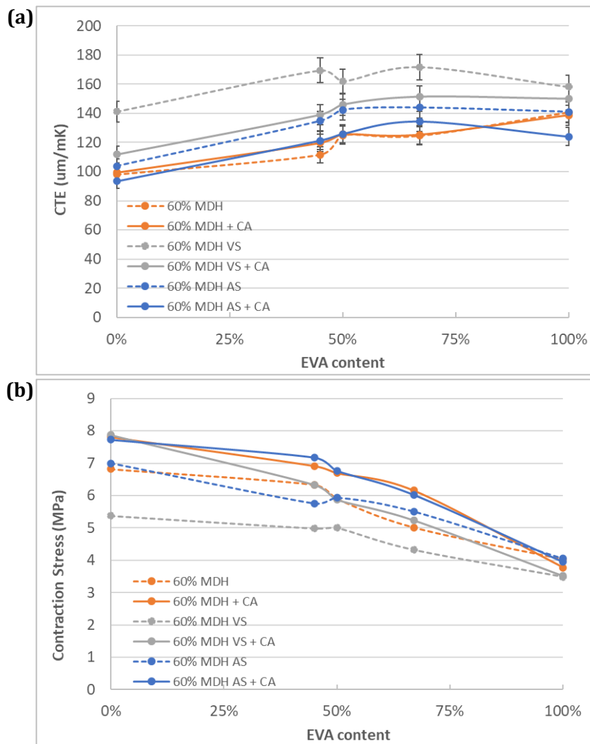
Figure 60 Coefficient of thermal expansion (a) and contraction stress (b) of EVA/LLDPE blends filled with 60 % of uncoated, vinylsilane (VS) and aminosilane (AS) coated magnesium-di-hydroxide (MDH), with and without coupling agent (CA)
