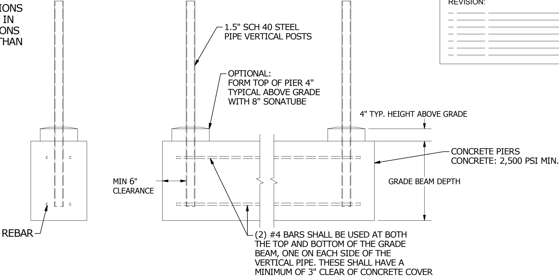
GRADE BEAM FOUNDATION DETAIL
