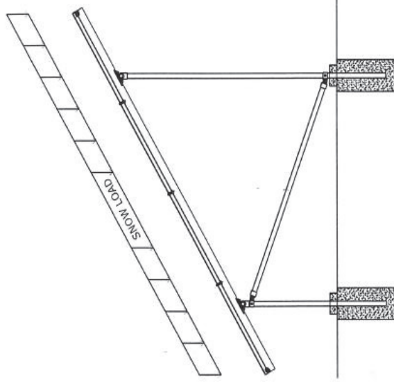
Snow Loading Diagram
