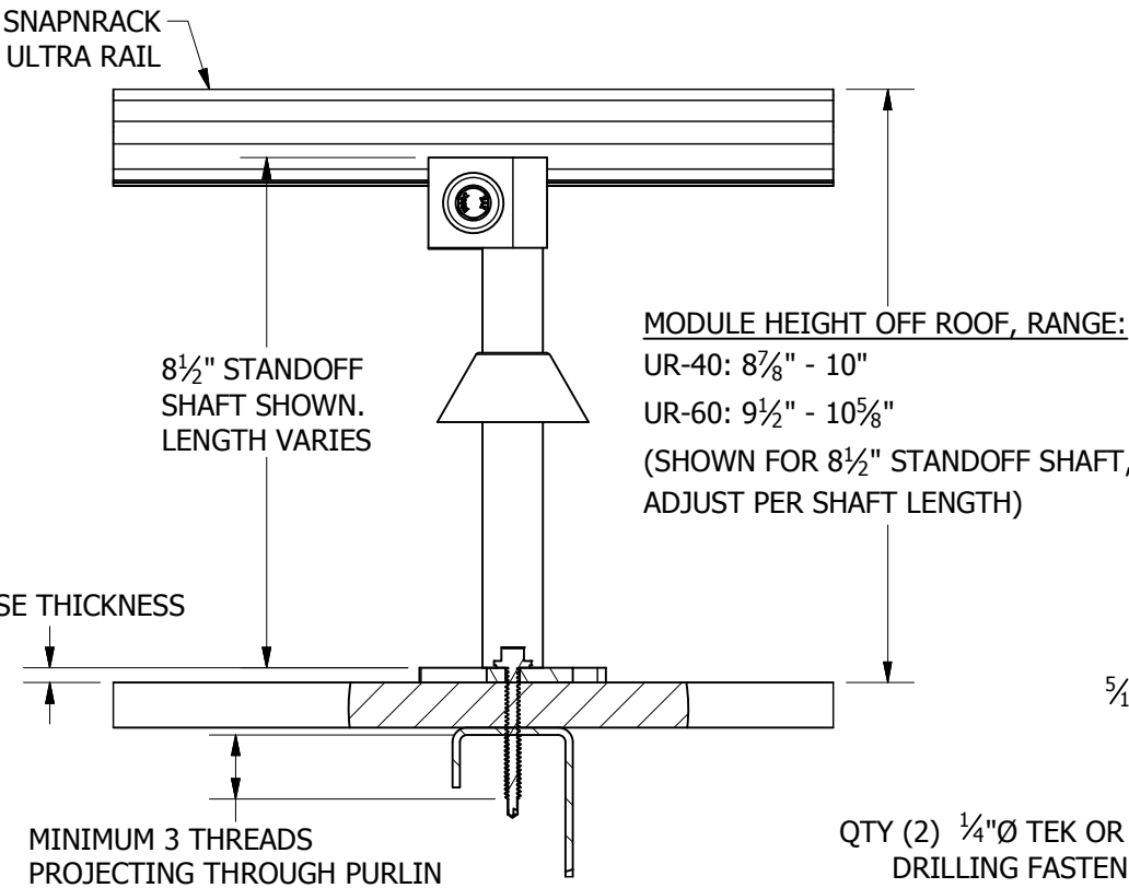
PENETRATION DETAIL
