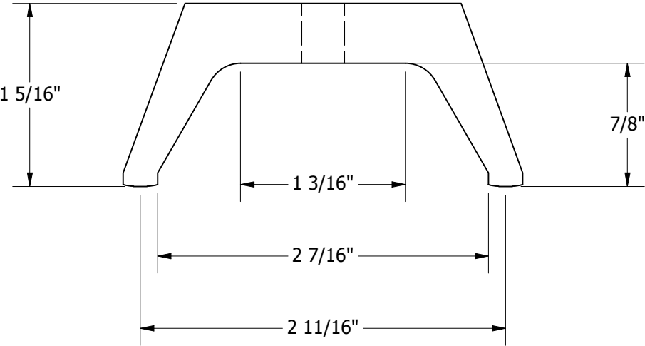
PART DIMENSIONS
