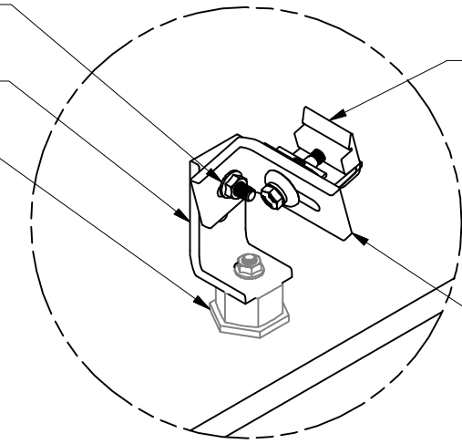
DETAIL A FRONT LEG, VARIABLE TILT WITH L FOOT (RAIL HIDDEN)
