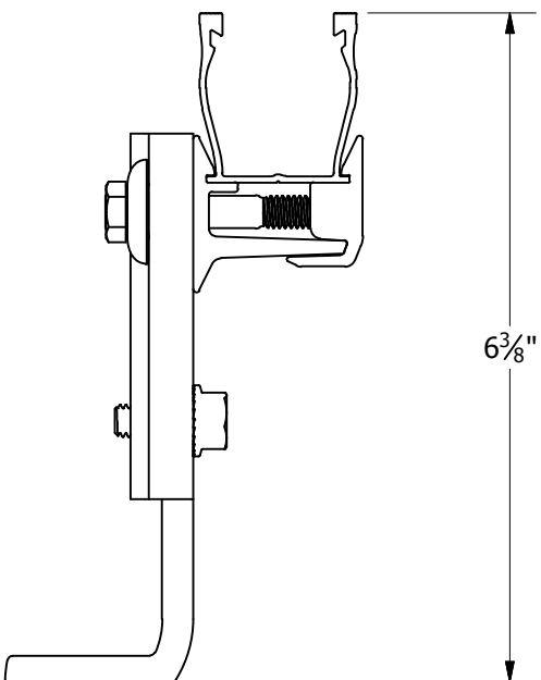
RAIL HEIGHT = 6 3/8" ABOVE ROOF SURFACE QTY. 1 L-FOOT, HIGH SLOT QTY. 1 EXTENSION, HIGH SLOT
