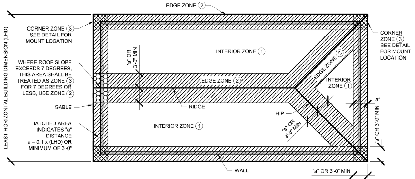
Figure 1: Roof Edge and Corner Zones
