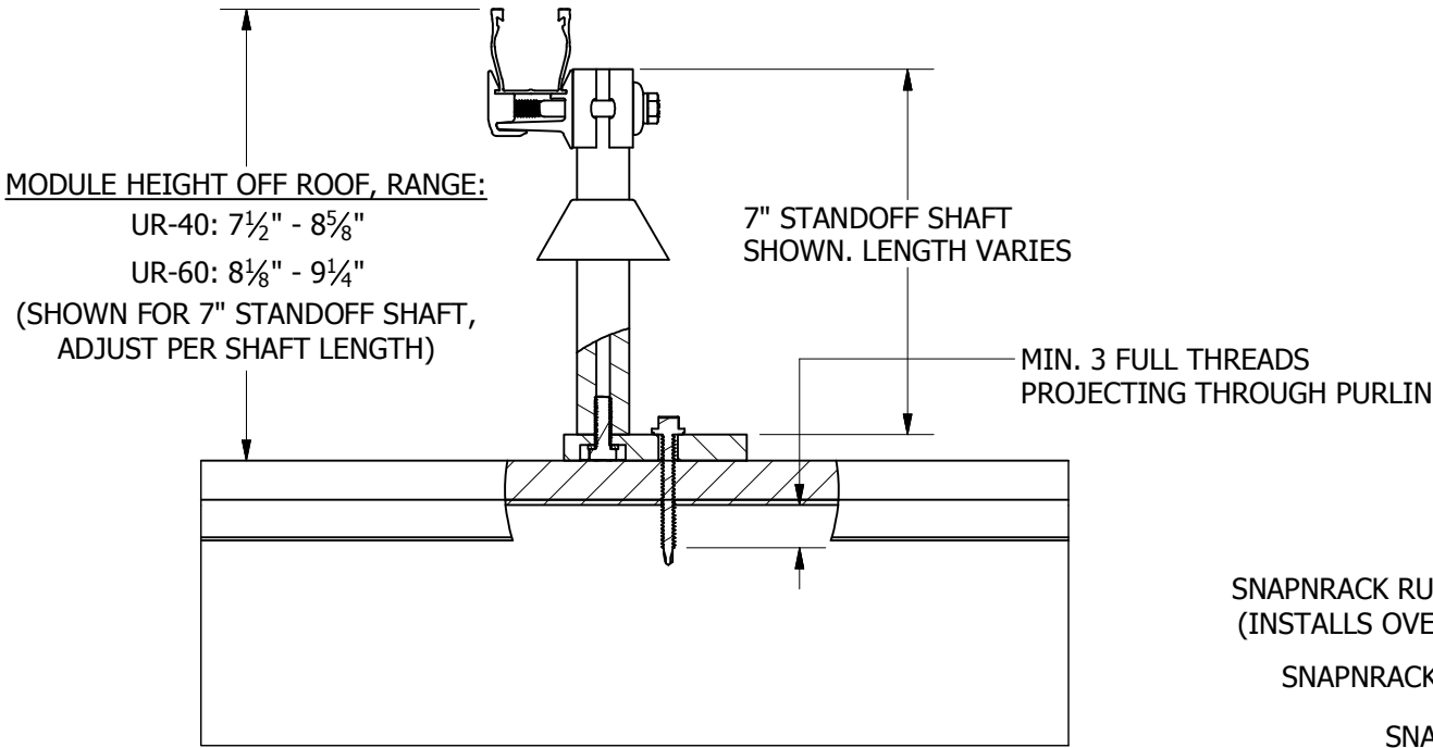
PENETRATION DETAIL
