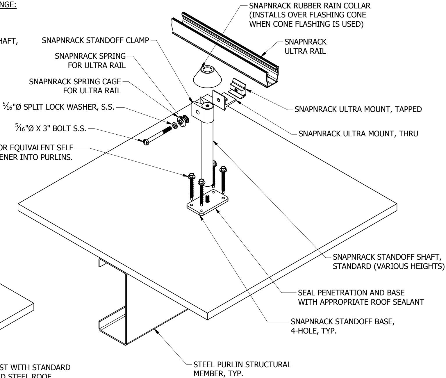
EXPLODED
