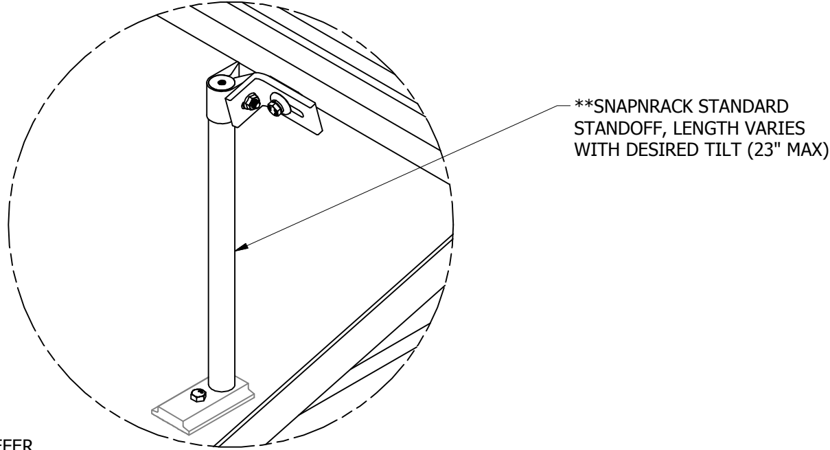
DETAIL B REAR LEG, FIXED TILT
