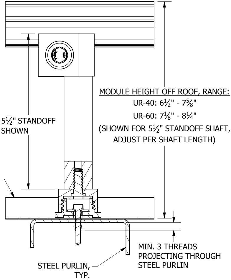
PENETRATION DETAIL
