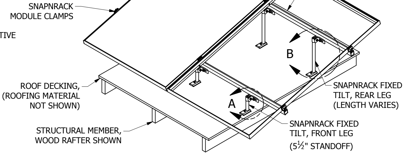
FIXED TILT, INSTALLED
