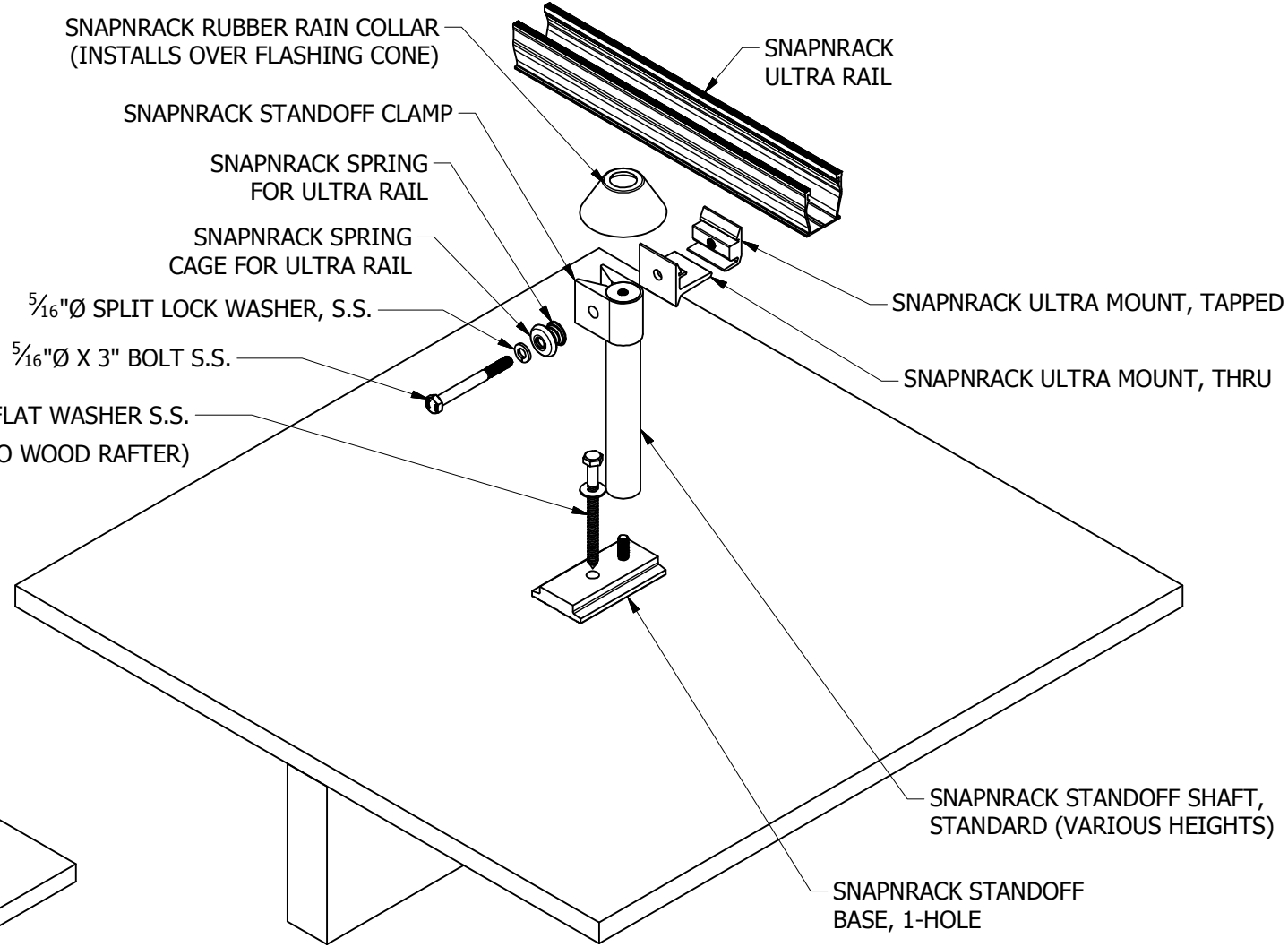
EXPLODED
