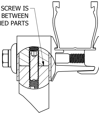
DETAIL A: SET SCREW PLACEMENT
