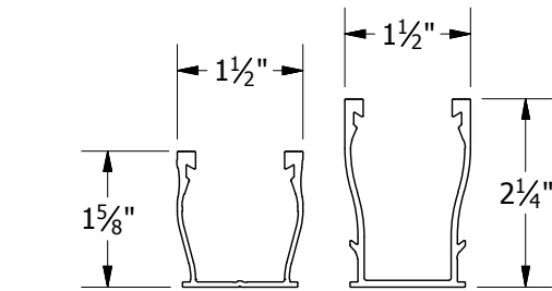
UR-40 RAIL | UR-60 RAIL FOR USE WITH SNAPNRACK ULTRA SERIES RAILS
