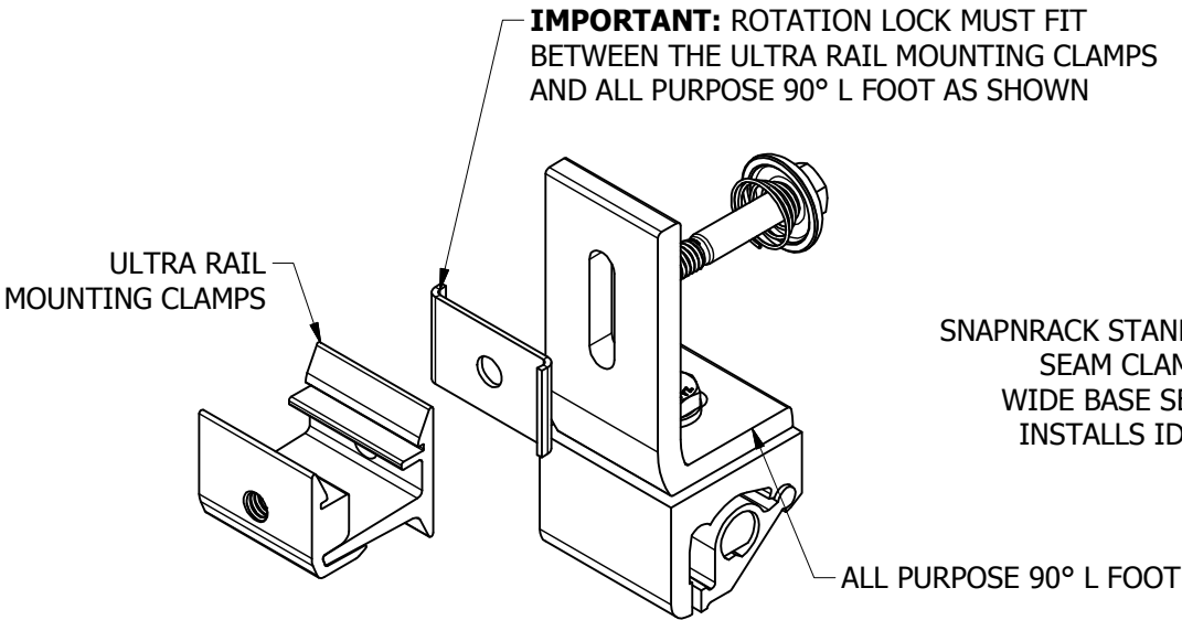
ROTATION LOCK ASSEMBLY
