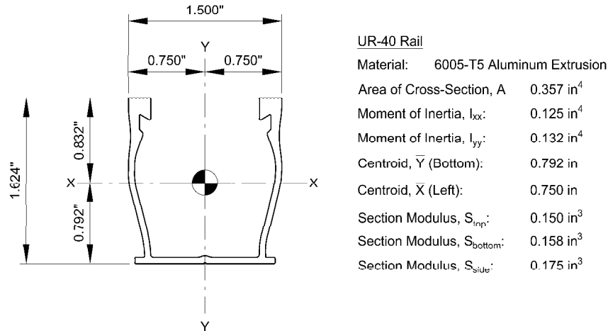
Figure 1: Diagram of UR-40 Rail Profile Covered by This Report (with Section Properties)
