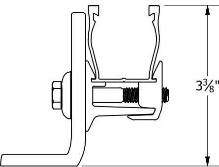
RAIL HEIGHT = 3 3/8" ABOVE ROOF SURFACE QTY. 1 L-FOOT, LOW SLOT
