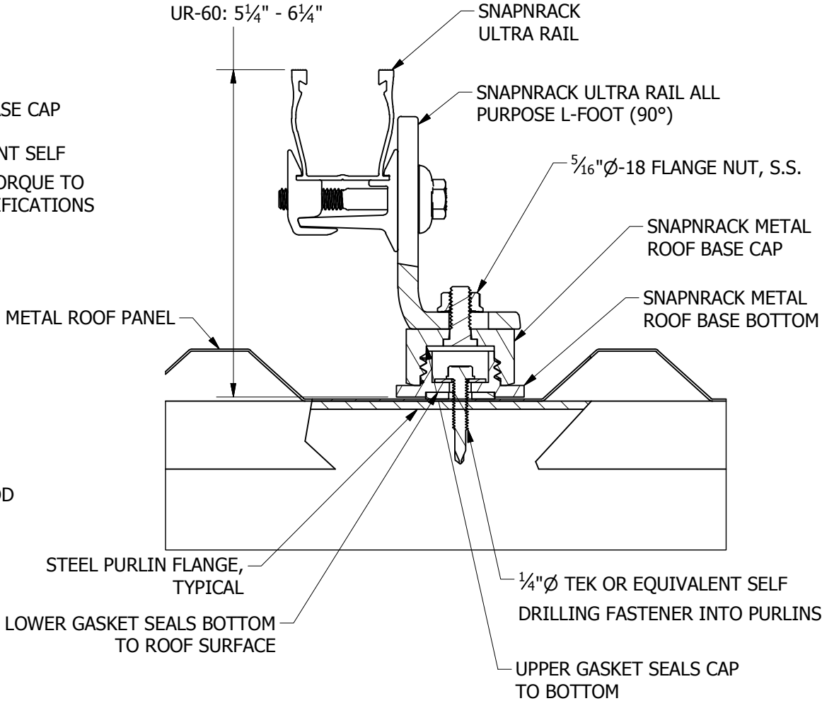
PENETRATION DETAIL
