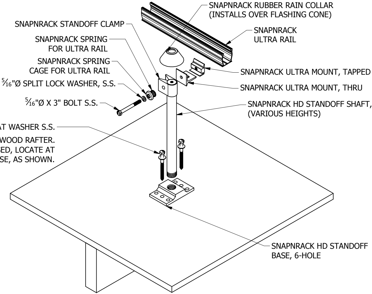
EXPLODED
