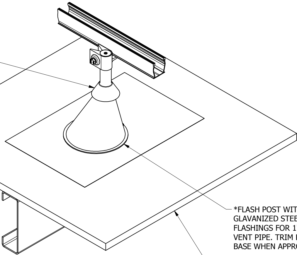
PENETRATION DETAIL
