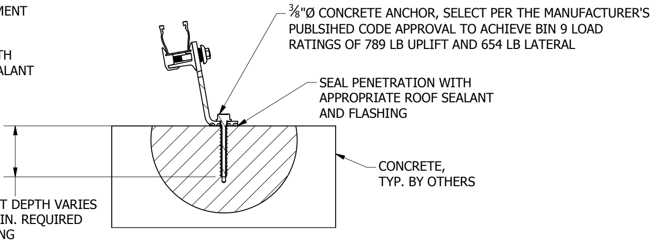
PENETRATION DETAIL: CONCRETE
