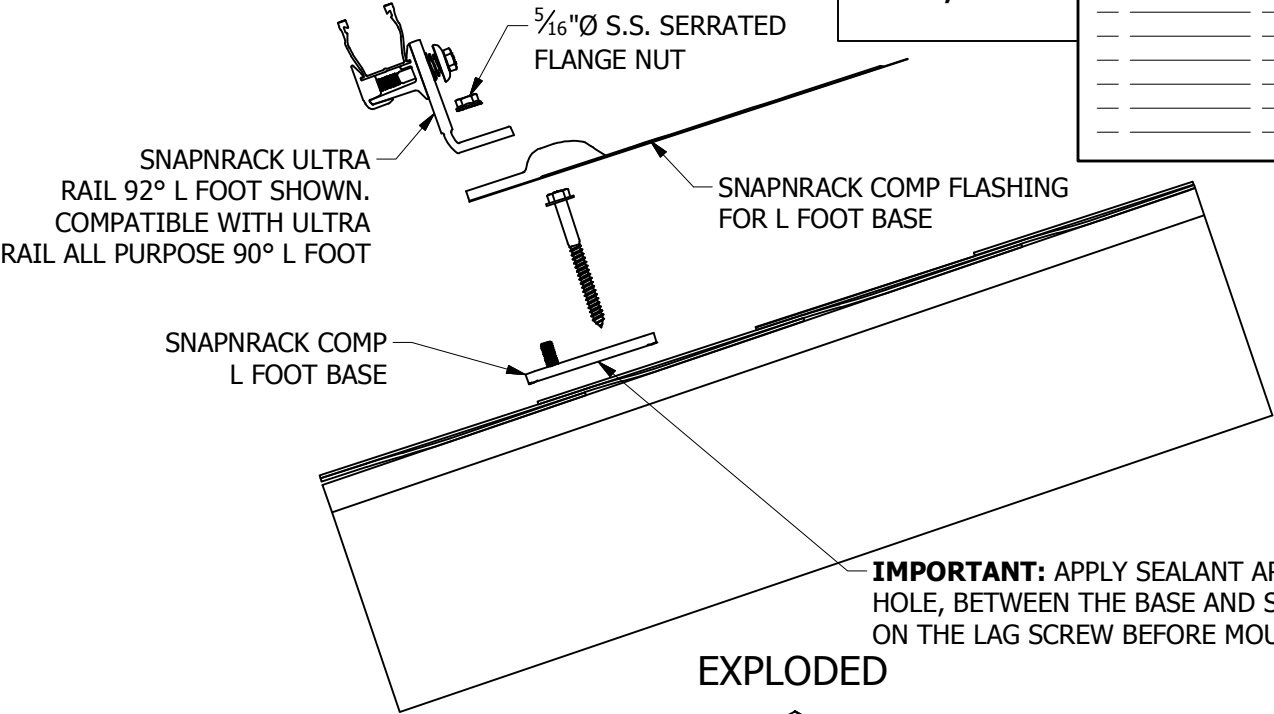
ULTRA RAIL 92° L FOOT: BIN 3
