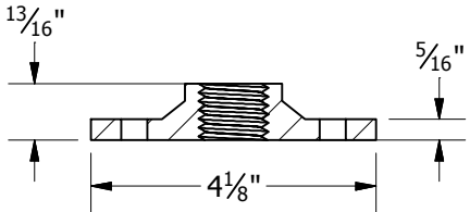
6-HOLE BASE, CROSS SECTION
