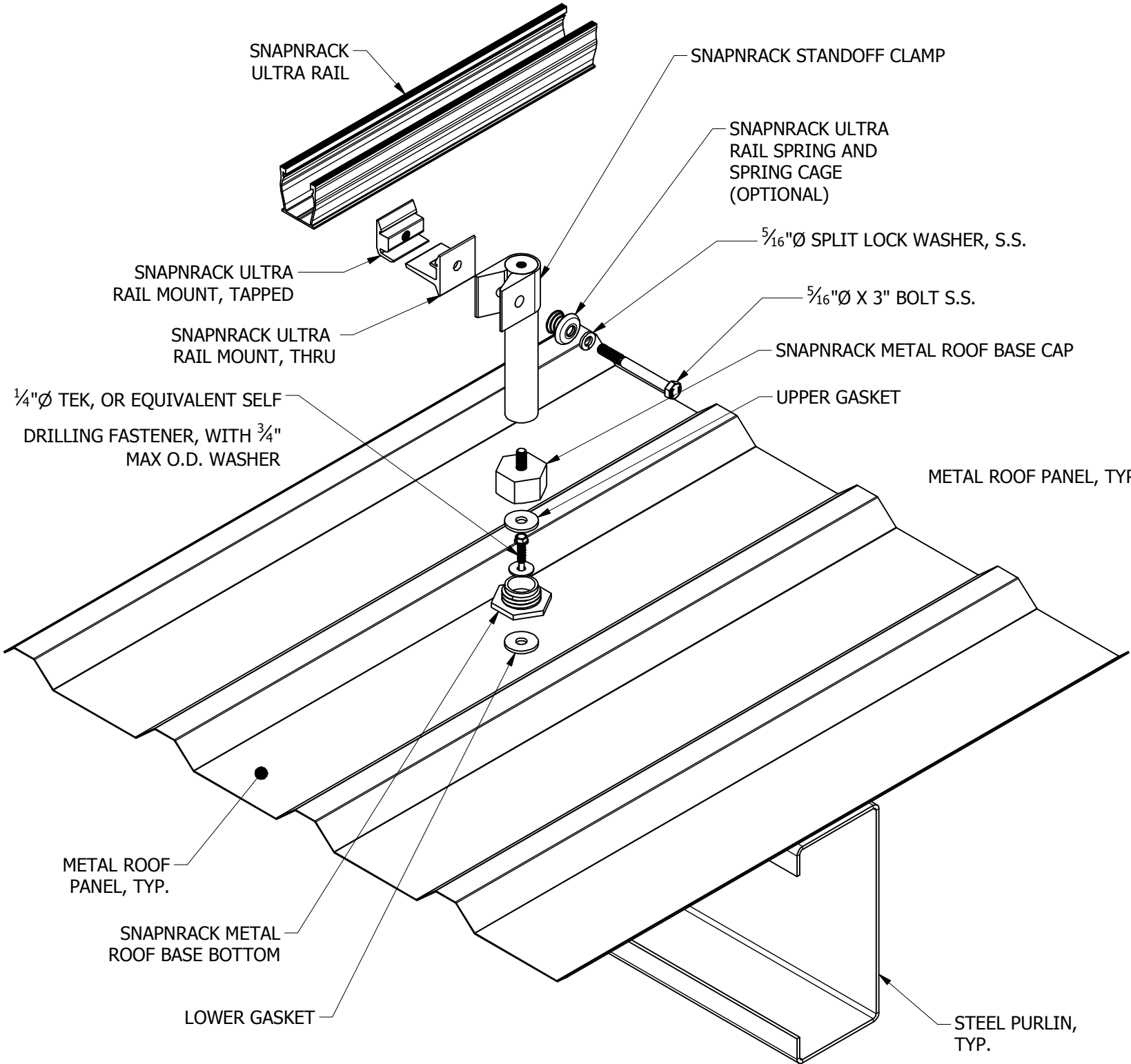
ULTRA RAIL METAL ROOF BASE, EXPLODED
