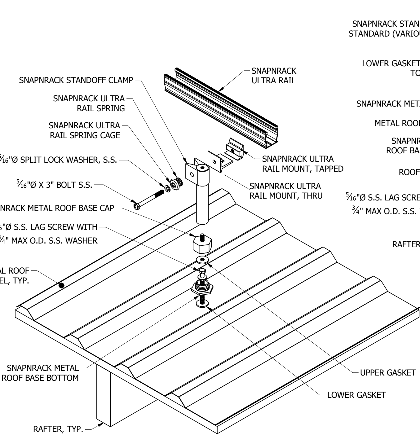
MRB SYSTEM INSTALLED, EXPLODED
