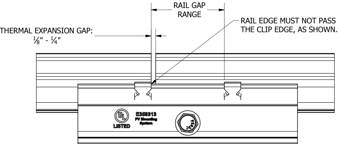
SPLICE ALIGNMENT LIMITS
