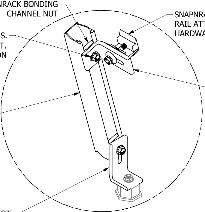
DETAIL B REAR LEG, VARIABLE TILT WITH L FOOT (RAIL HIDDEN)
