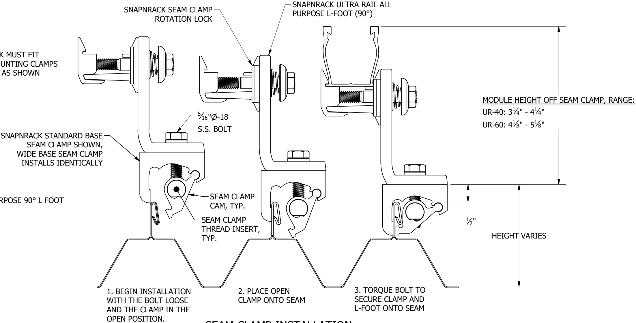
SEAM CLAMP INSTALLATION
