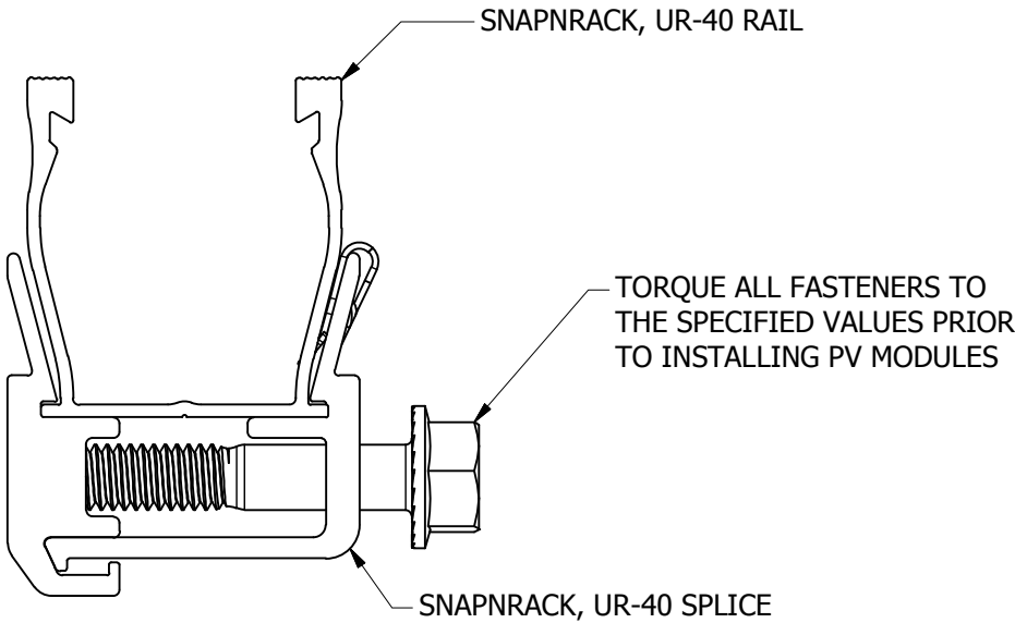
SNAPNRACK, UR-40 SPLICE INSALLED
