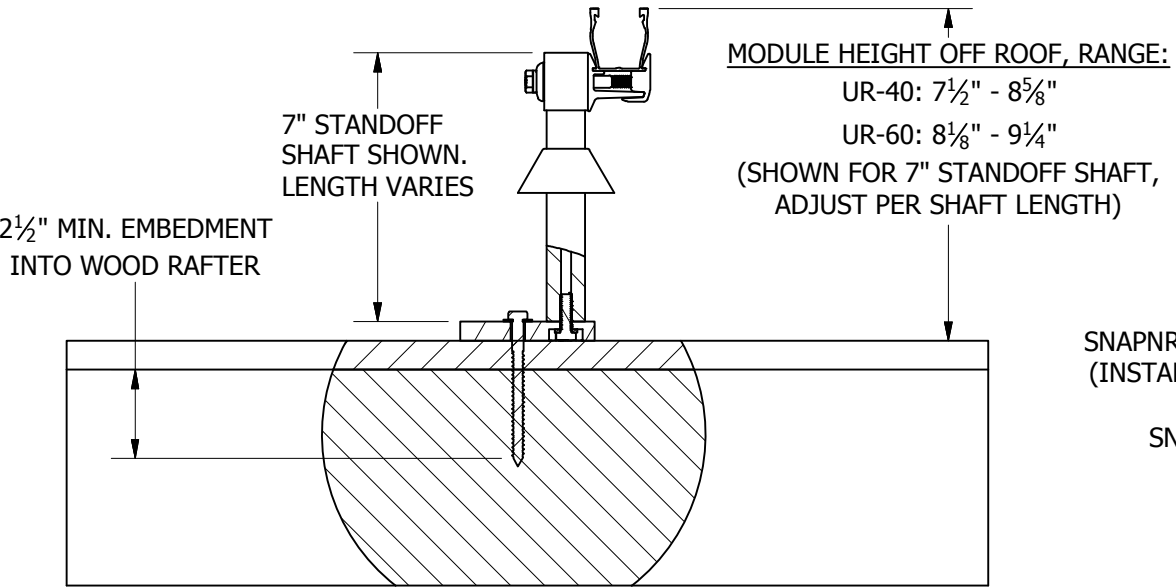
PENETRATION DETAIL
