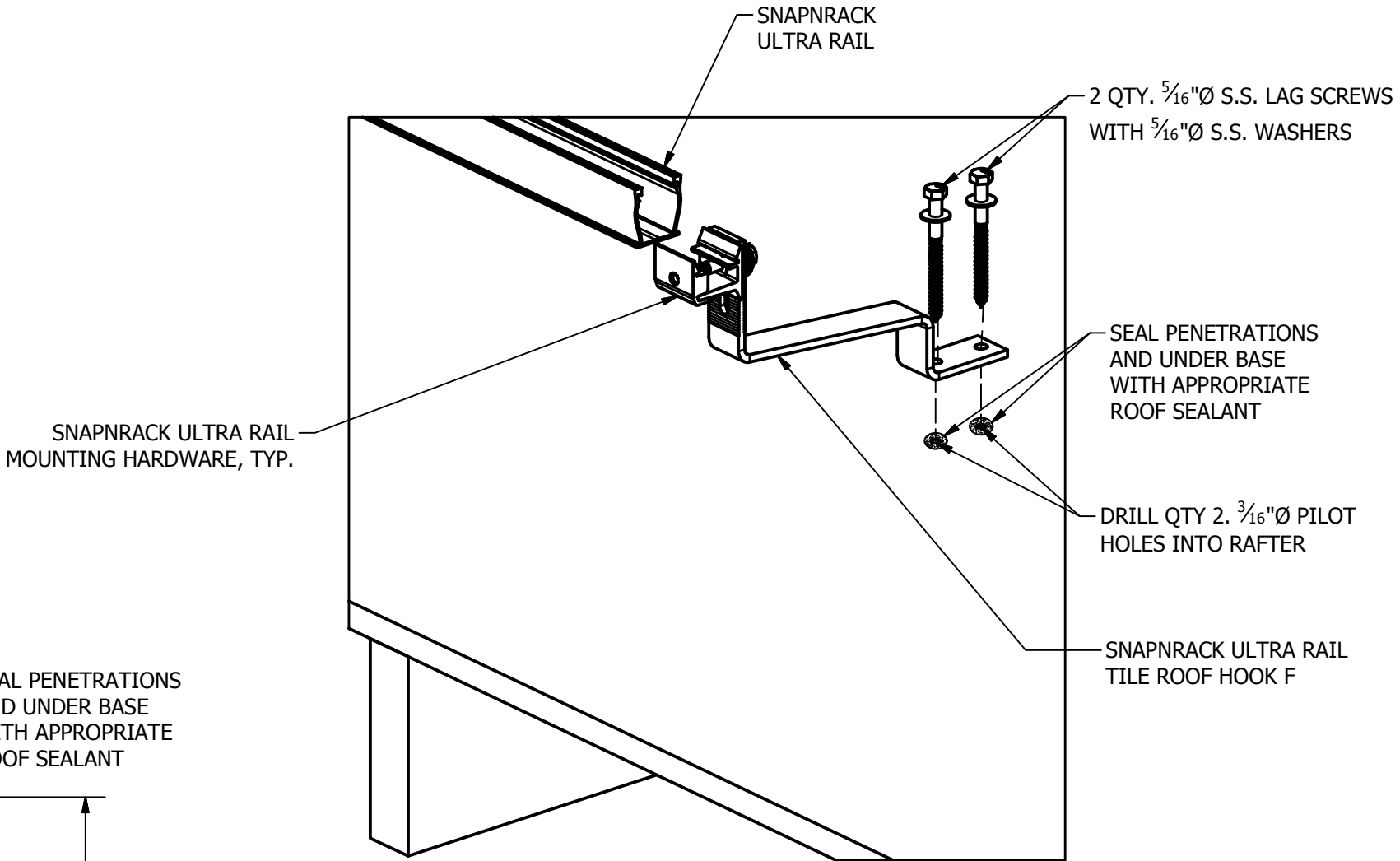
ULTRA RAIL TILE ROOF HOOK F, EXPLODED
