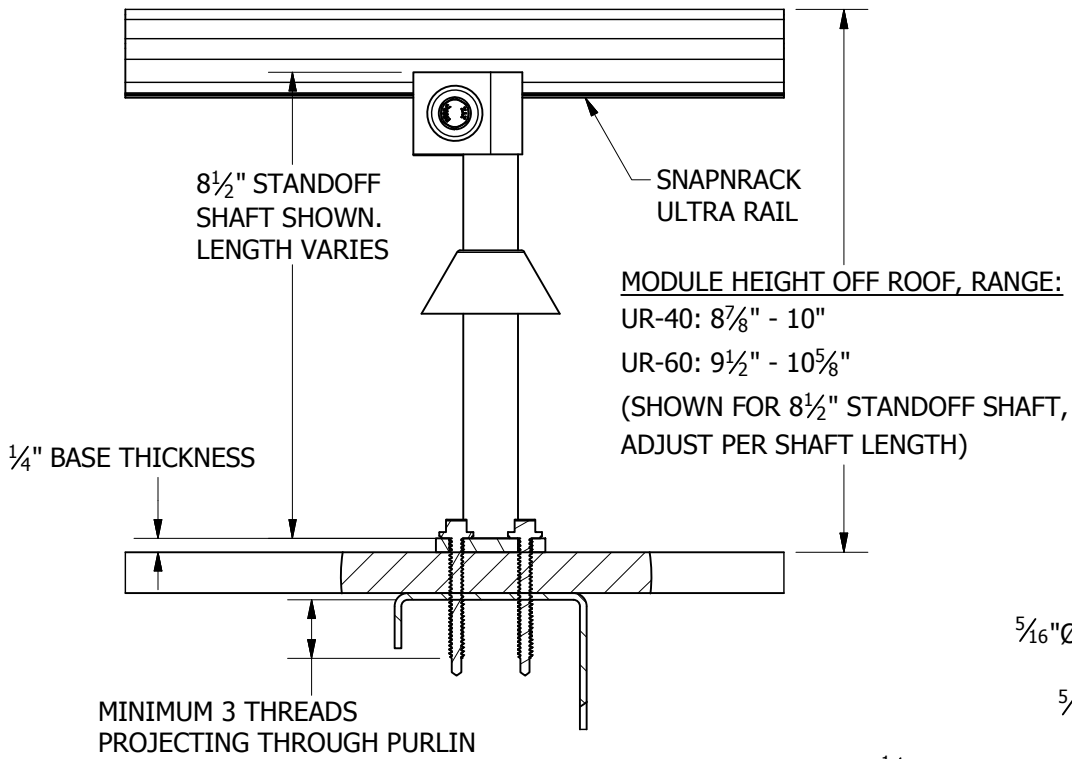
PENETRATION DETAIL
