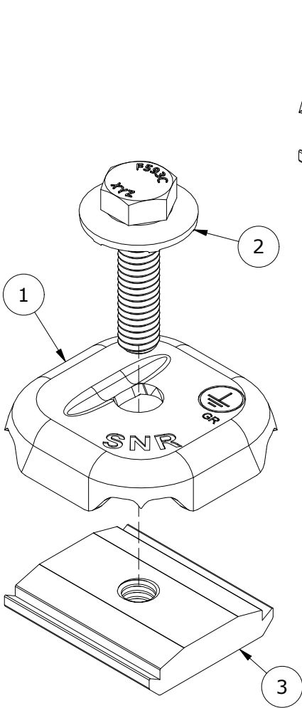
EXPLODED VIEW
