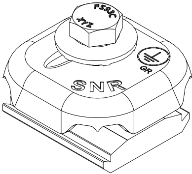
ASSEMBLED VIEW
