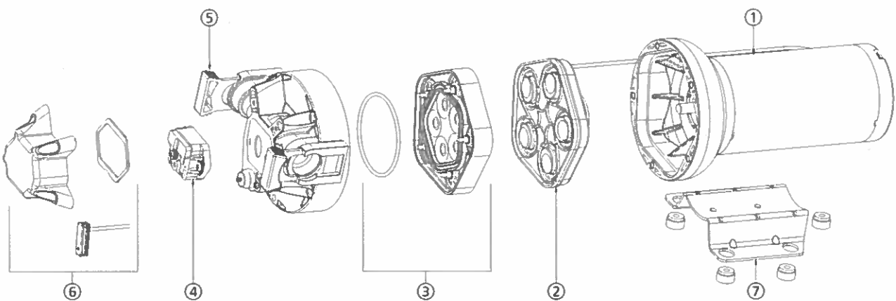
Exploded View
