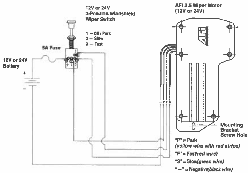
Wiring Diagram #1 (for normal two-speed operation)
