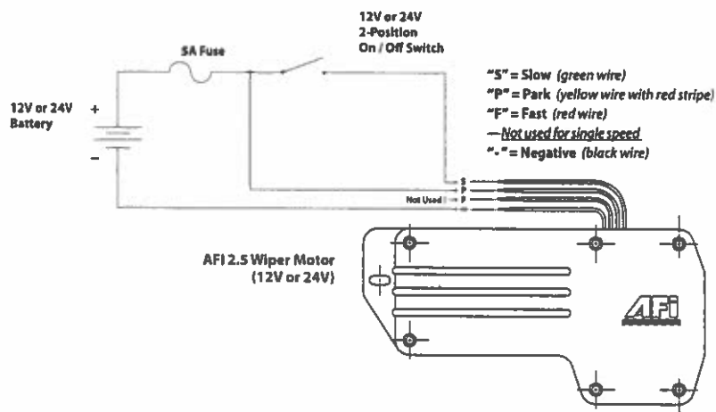
Wiring Diagram #2 (for optional one-speed operation)
