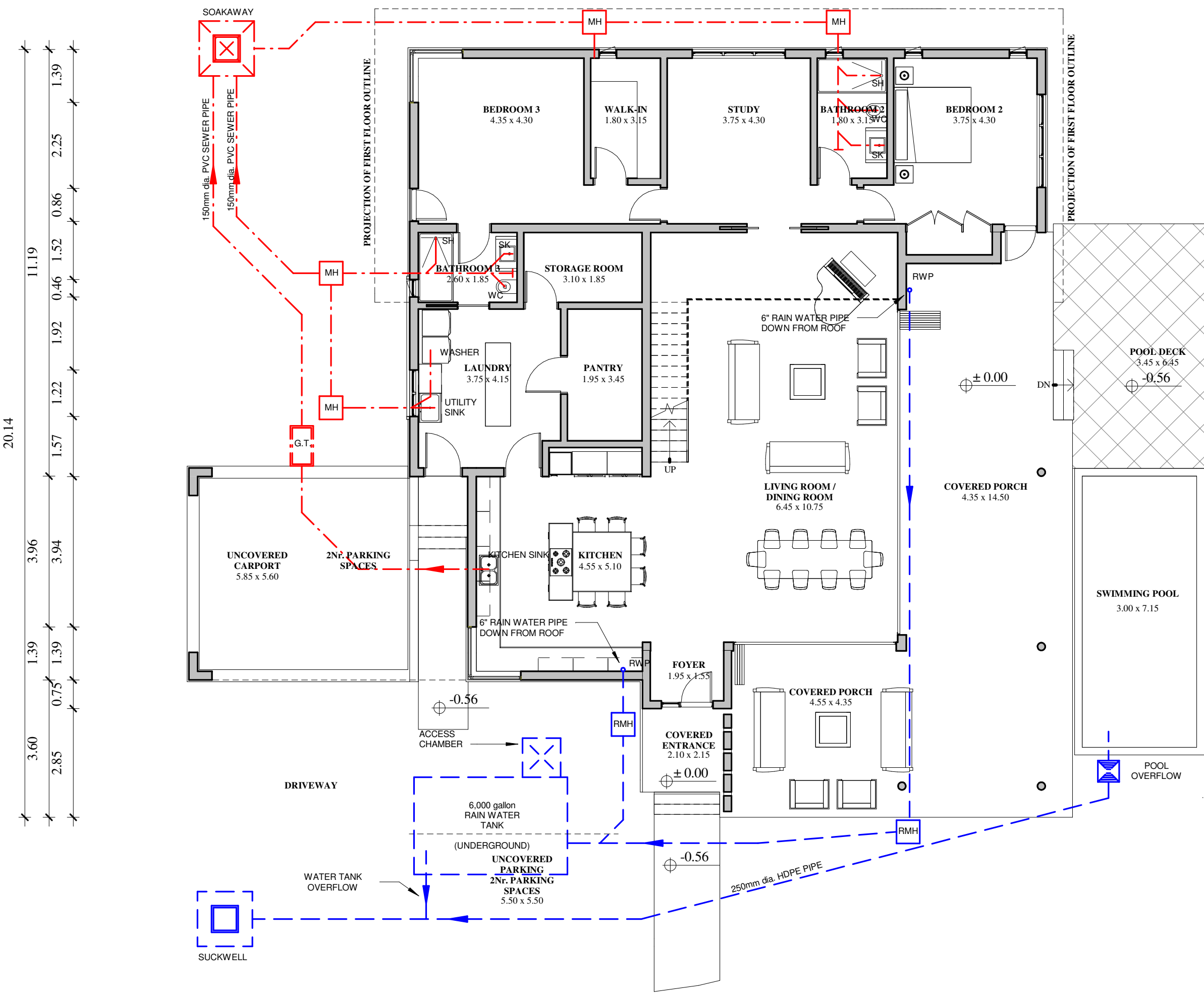
PROJECTION OF FIRST FLOOR OUTLINE
