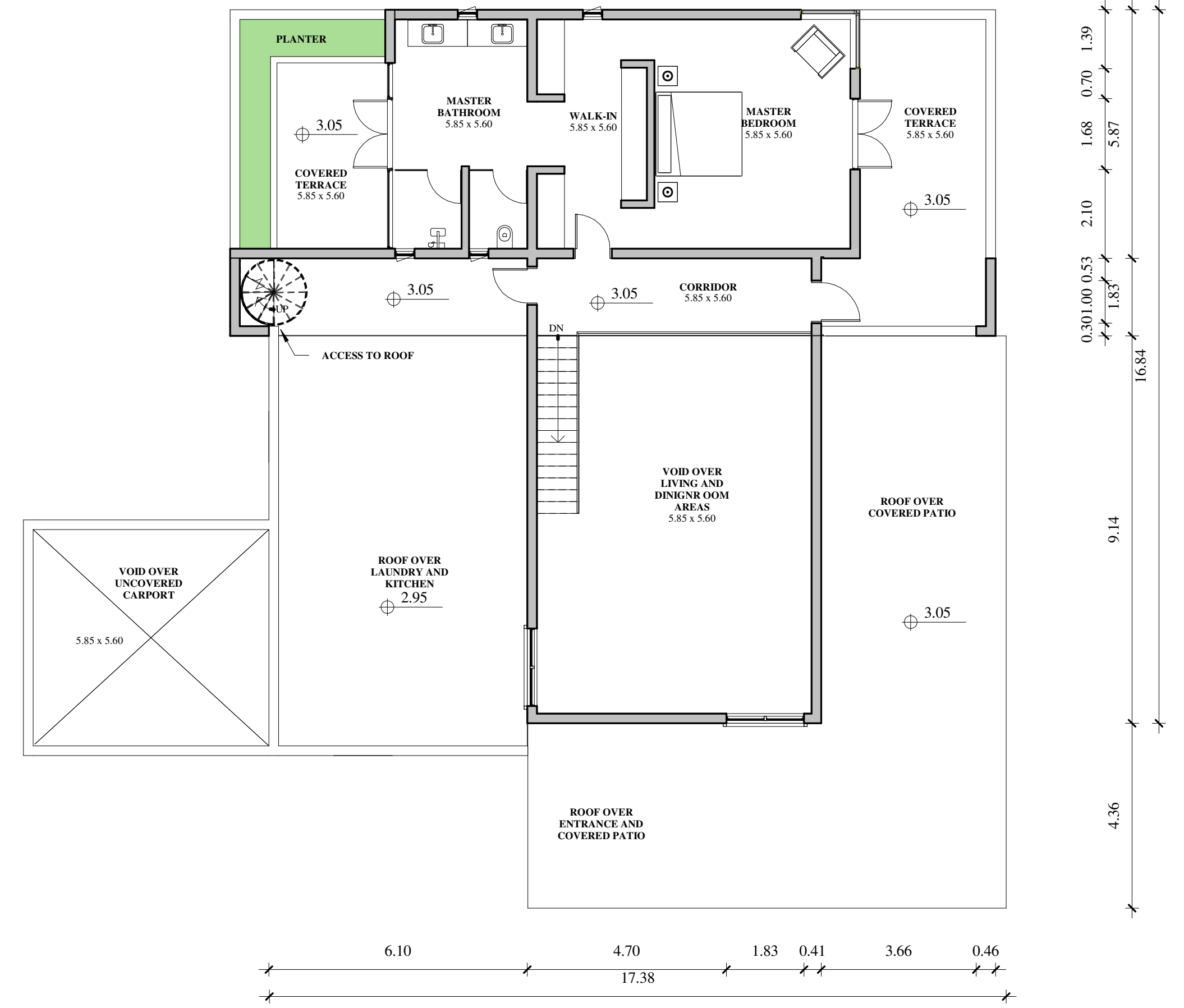
2 FIRST FLOOR LAYOUT COVERED AREA: 134.03 m 2 1 : 100
