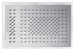
K022 frame: 50 x 35 cm showerhead: 45 x 30 cm rain / toning jet
