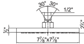
ART. 8026U Shower head with anti-limestone nozzles / Rociador anticalcáreo duche
