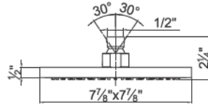
ART. 8008U Shower head with anti-limestone nozzles / Rociador anticalcáreo duche
