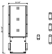
EXAMPLE OF CONFIGURATION - 3 OUTLETS
