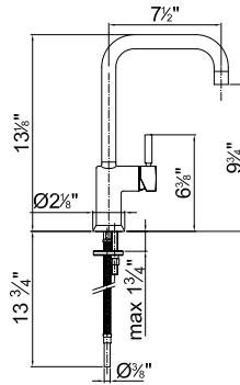
ART. 1854U Sink mixer / Monomando fregadera
