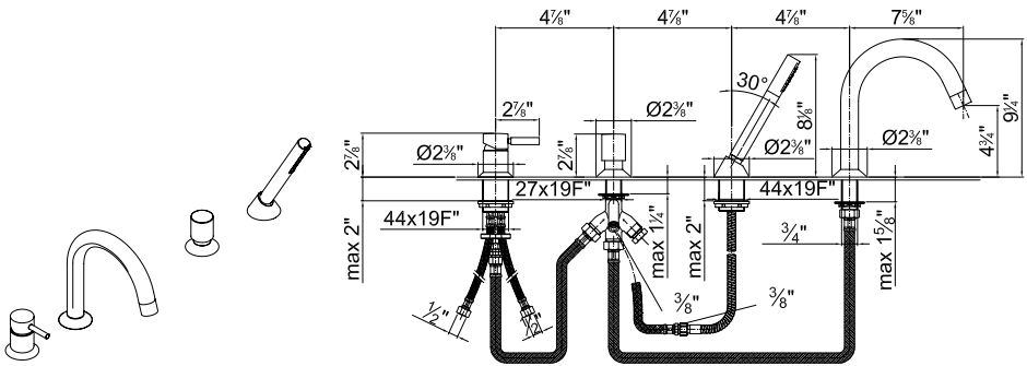
ART. 1865U Bath-side group / Bateria horizontal bañera
