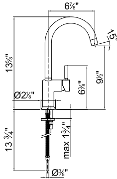
ART. 1855U Sink mixer / Monomando fregadera
