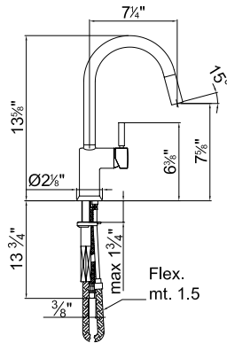
ART. 1852U Sink mixer / Monomando fregadera
