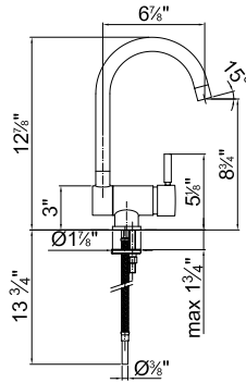
ART. 1859U Sink mixer / Monomando fregadera
