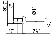
Wall-mount spout / Caño a pared
