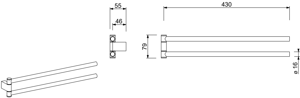
ART. 7682 Porta salviette snodato / Swivel towel rail / Porte-serviettes pivotant / Schwenkbarer Handtuchhalter / Toallero giratorio
