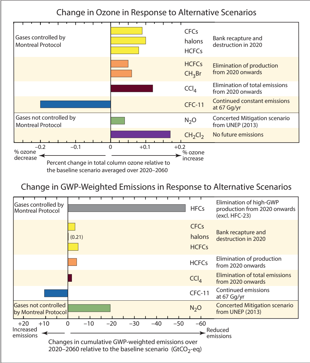
Figure ES-9. Changes in ozone and GWP-weighted emissions for a selection of alternative scenarios. Changes in total column ozone (upper panel) and GWP-weighted emissions (lower panel) that occur in the alternative scenarios as described in the figure. The values are differences in average ozone (top panel) over the period 2020–2060 and cumulative GWP-weighted emission (lower panel) over the same period between the alternative scenarios and the baseline scenario. A decrease in total ozone and an increase in GWP-weighted emissions occur when the alternative scenario emissions are higher than in the baseline scenario. Numerical values of these changes are shown in Table 6-5. Note that the change resulting from the elimination of HFC production shown in the lower panel is not shown in the upper panel because HFCs play such a small role in the chemical destruction of ozone. Chemical terms used in the figure are methyl bromide (CH 3 Br), carbon tetrachloride (CCl 4 ), nitrous oxide (N 2 O), and dichloromethane (CH 2 Cl 2 ). [Also Figure 6-1]
