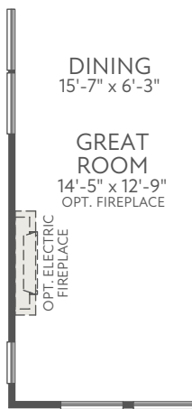
FIRST FLOOR EXTERIOR STYLE L AT END UNIT CONDITION GARAGE SIDE
