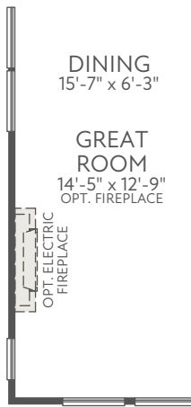
FIRST FLOOR EXTERIOR STYLE J AT END UNIT CONDITION GARAGE SIDE
