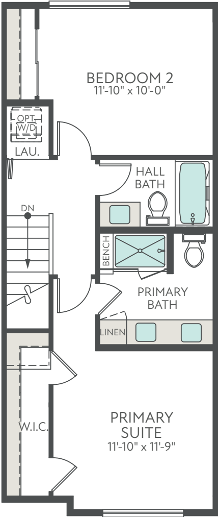
THIRD FLOOR
