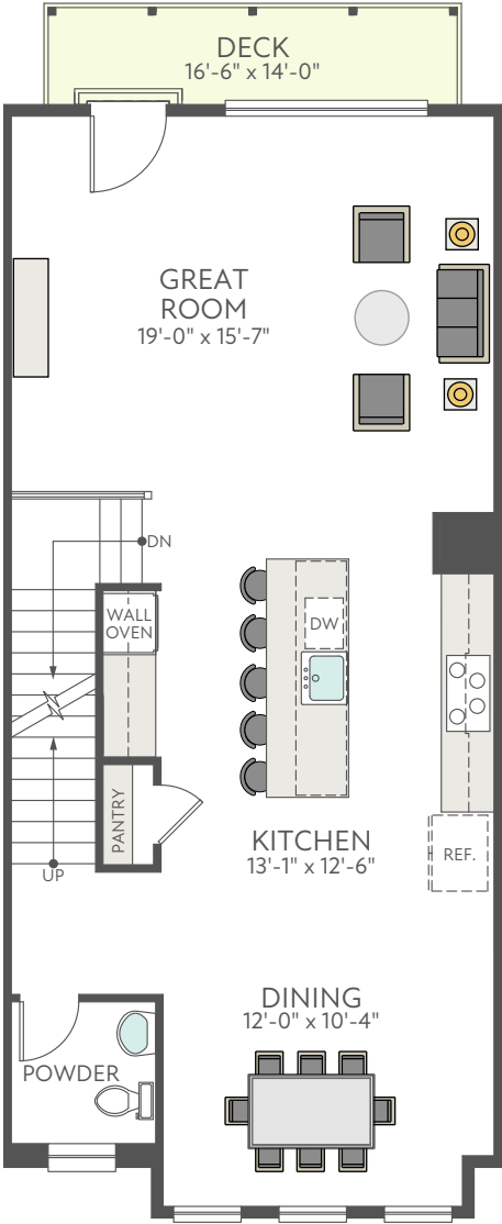
FIRST FLOOR
