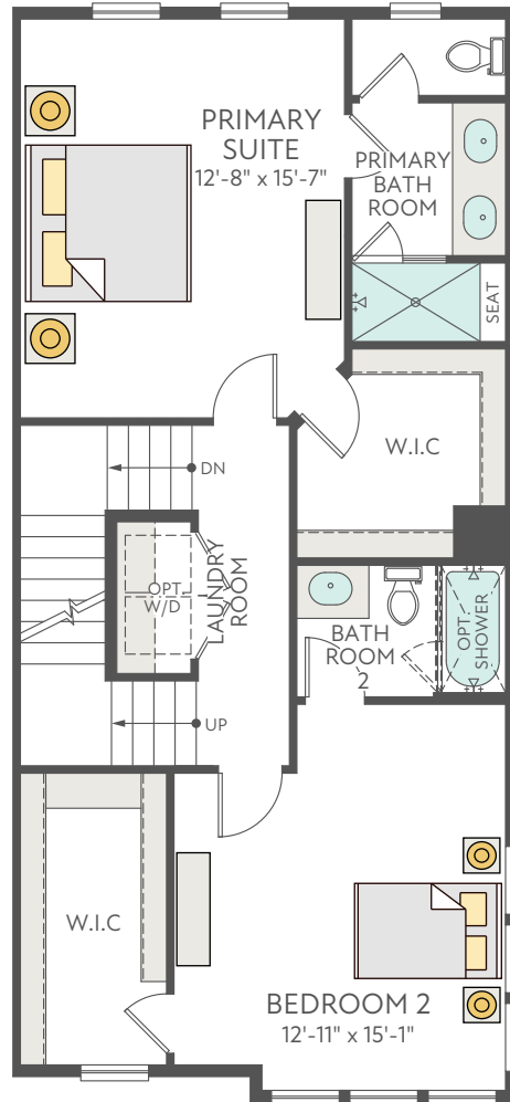
SECOND FLOOR
