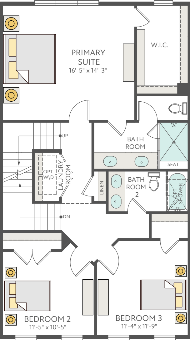
THIRD FLOOR
