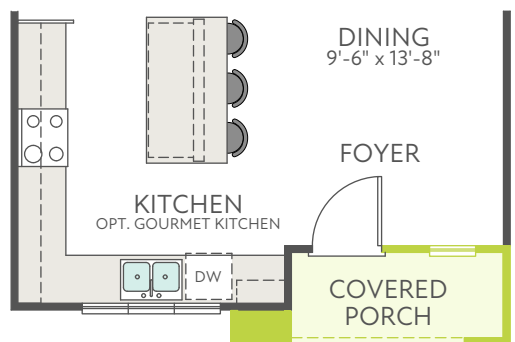
FIRST FLOOR EXTERIOR STYLE L
