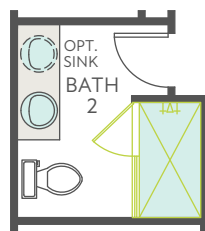
OPT. SHOWER AT BATH 2
