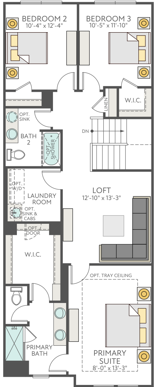
SECOND FLOOR EXTERIOR STYLE I
