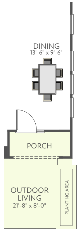
FIRST FLOOR EXTERIOR STYLE D AT PORCH SIDE END UNIT
