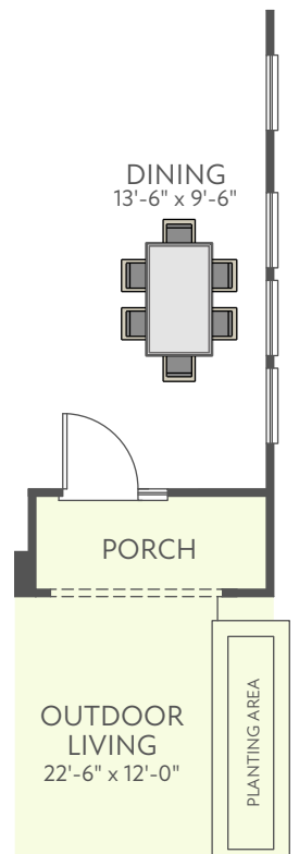
FIRST FLOOR EXTERIOR STYLE C AT PORCH SIDE END UNIT
