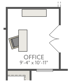
OPT. OFFICE ILO FLEX
