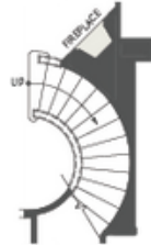
OPT. FIREPLACE
