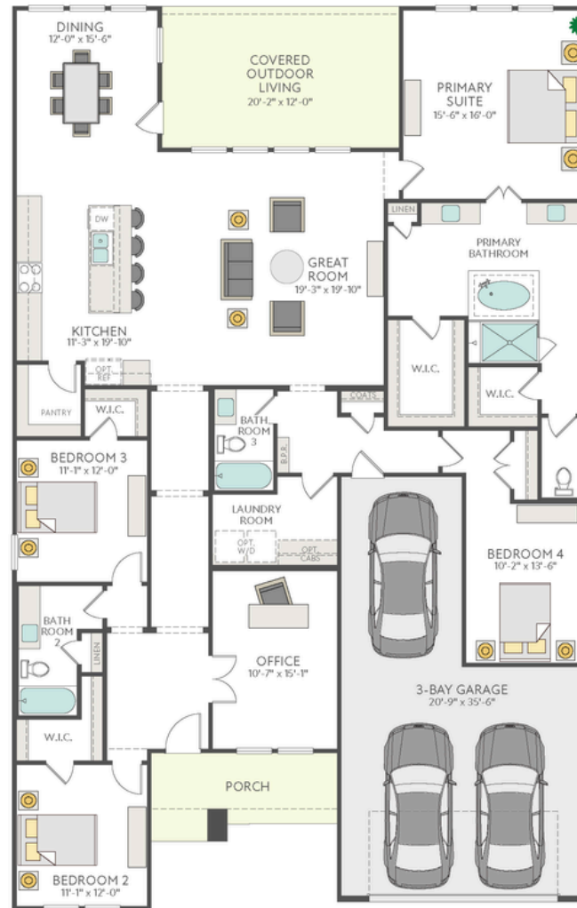
Floor Plan
