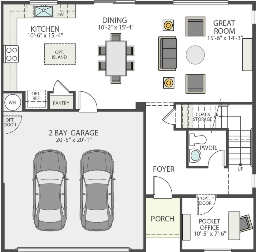
FIRST FLOOR
