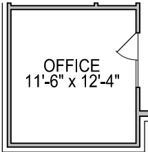
FIRST FLOOR PLAN OPT. #0569 OFFICE FROM FLEX
