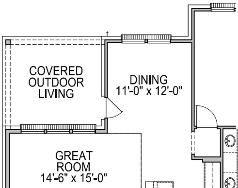
FIRST FLOOR PLAN OPT. #0105 COVERED OUTDOOR LIVING
