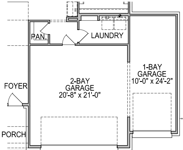
FIRST FLOOR PLAN OPT. #0593 1 BAY GARAGE
